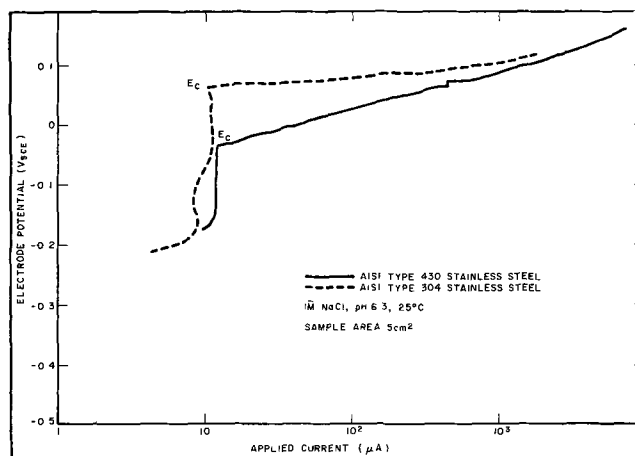
Fig. 3. Potentiodynamic anodic-polarization curves for steels exposed to oxygen-saturated 1M NaCl sweep rate, 0.600 V/hr.
